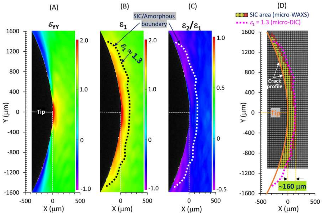
Figure 4. Spatial distribution of local strains around a crack tip. Two-dimensional distributions of (A) true strain \epsilon_{yy} in laboratory coordinate, (B) major principal true strain \epsilon_1 , and (C) strain biaxiality of principal strains \epsilon_2/\epsilon_1 for a pre-notched NR specimen subjected to an applied macroscopic tensile true strain of 0.62. The dotted line depicts the iso- \epsilon_1 line of \epsilon_1 = 1.3 . (D) Comparison between the SIC zone (as shown in Figure 2) identified by micro-beam WAXD measurements, and the area where \epsilon_1 > 1.3 , as determined by micro-DIC. The iso- \epsilon_1 line of \epsilon_1 = 1.3 closely parallels the boundary between SIC and amorphous states.
