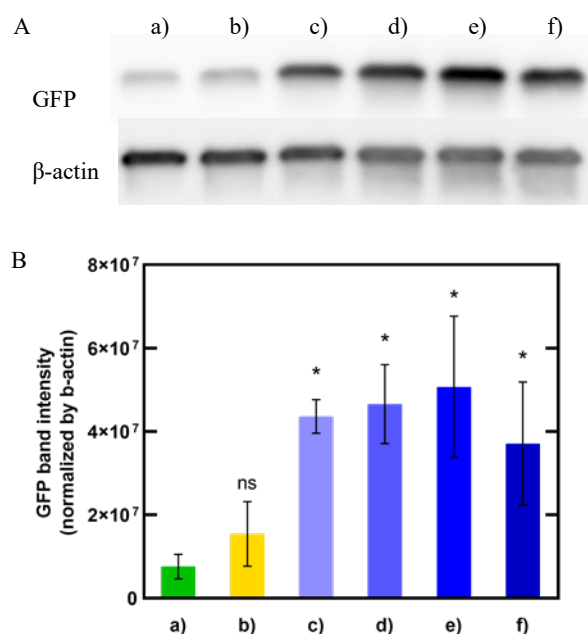
Fig. 2 A. Western blotting image of cell lysates after cellular internalization of a) Mt and b) Mt associated with cG, c) cGNS(50), d) cGNS(100), e) cGNS(200), and f) cGNS(400). B. Efficiency of cellular internalization of Mt and Mt associated with cG and cGNS. The value for the Mt group is 1. *, p < 0.05 ; significant difference from the Mt group, ns; not significant.
