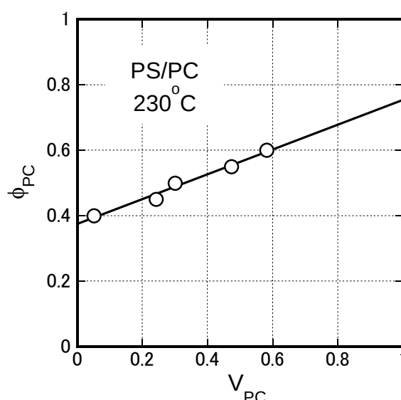
図 12 PS/PC の lever rule plot
