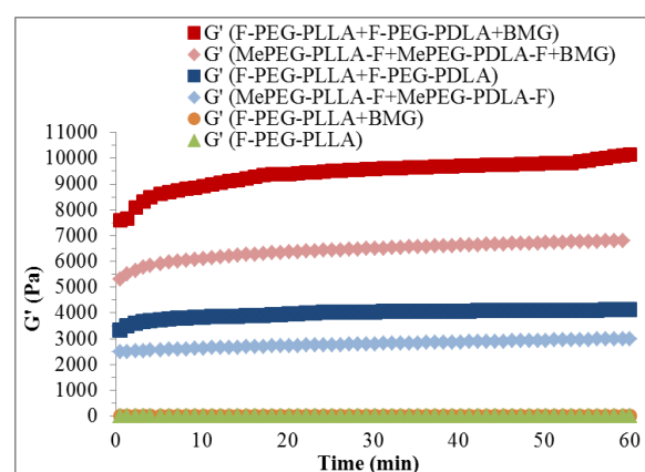
Figure 6. The time-dependent rheological changes for the mixed dispersions containing various copolymers in 20wt/wt% at 37°C.
