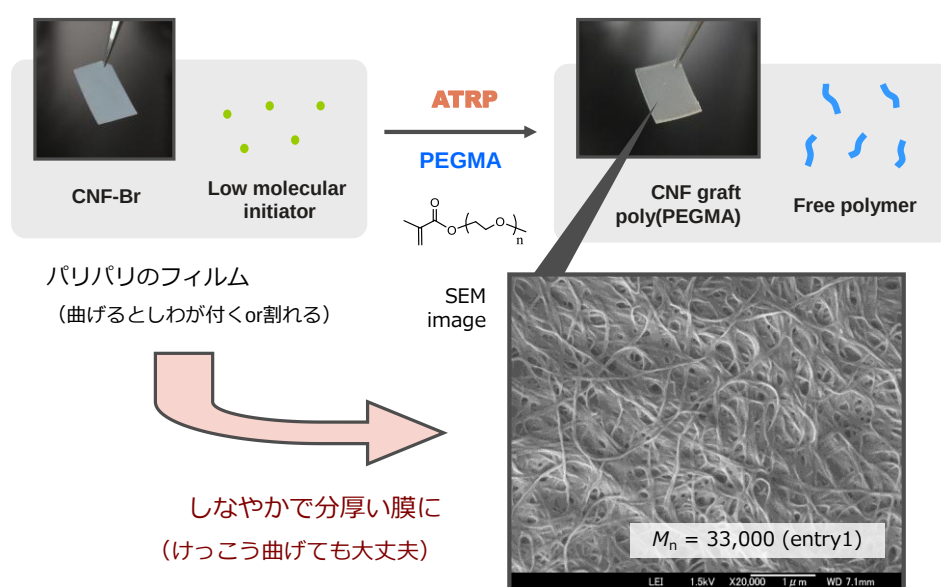
Figure 6 Fabrication of CNF non-woven sheet with concentrated brushes of hydrophilic polymers by surface-initiated ATRP.
